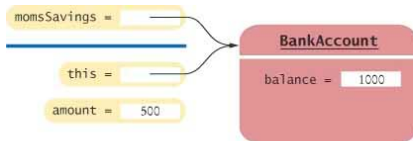
FIGURE 3-8 The Implicit Parameter of a Method Call
