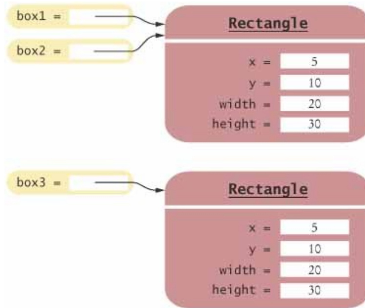
FIGURE 5-4 Comparing Object References
