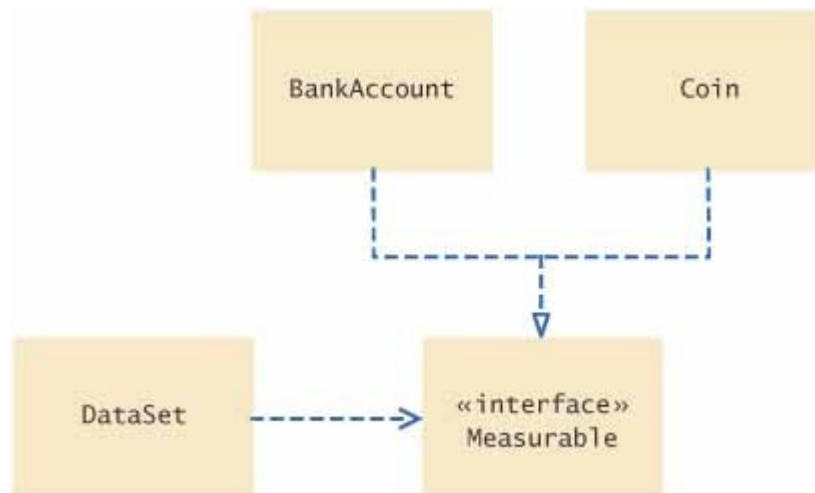
FIGURE 9-1 UML Diagram of the DataSet Class and the Classes that Implement the Measurable Interface
