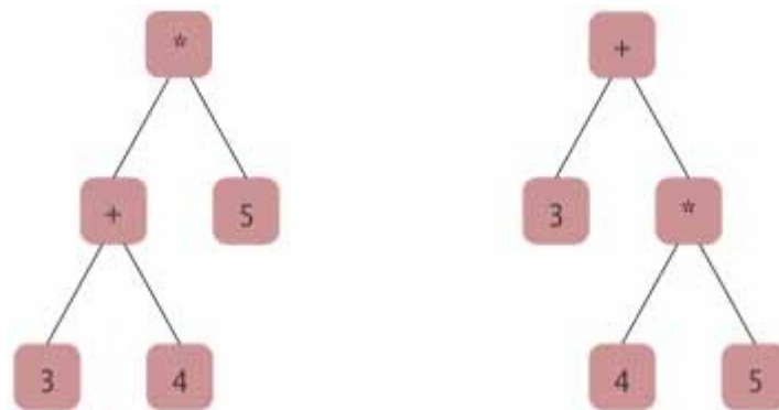
FIGURE 16-14 Expression Trees
