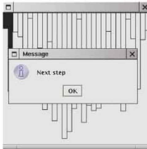
FIGURE 14-3 Graphical Animation
