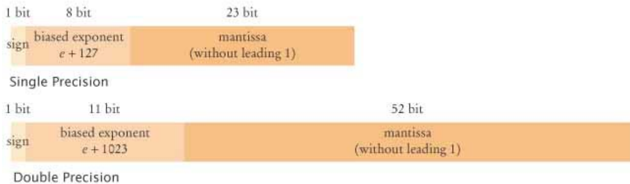
FIGURE K-1 IEEE Floating-Point Representation
