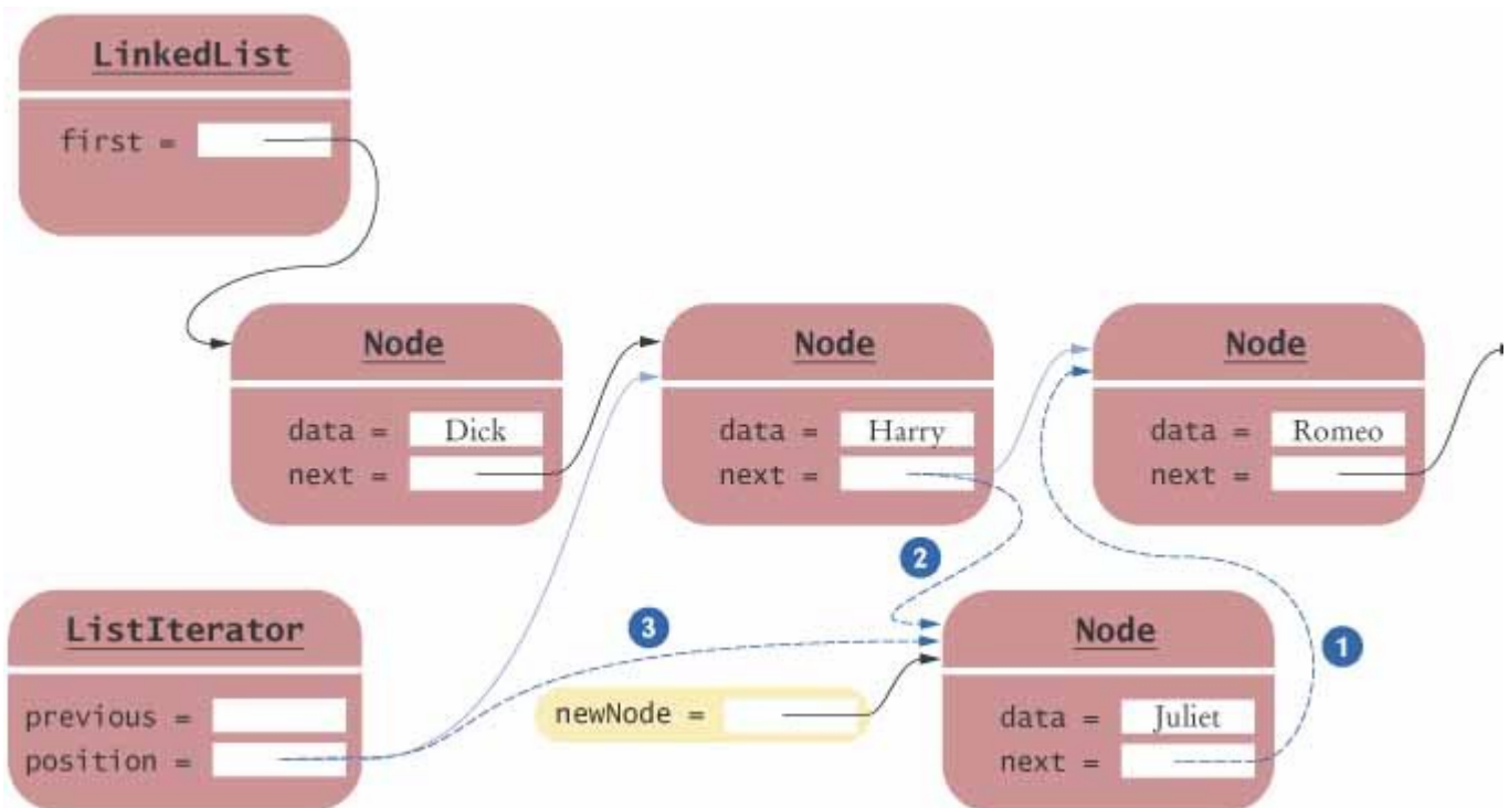
FIGURE 15-7 Adding a Node to the Middle of a Linked List
