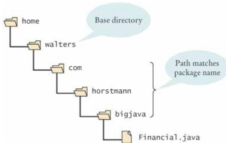
FIGURE 8-5 Base Directories and Subdirectories for Packages
