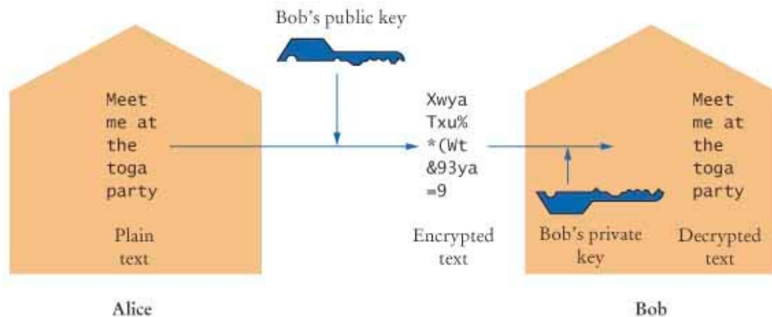
Public Key Encryption
