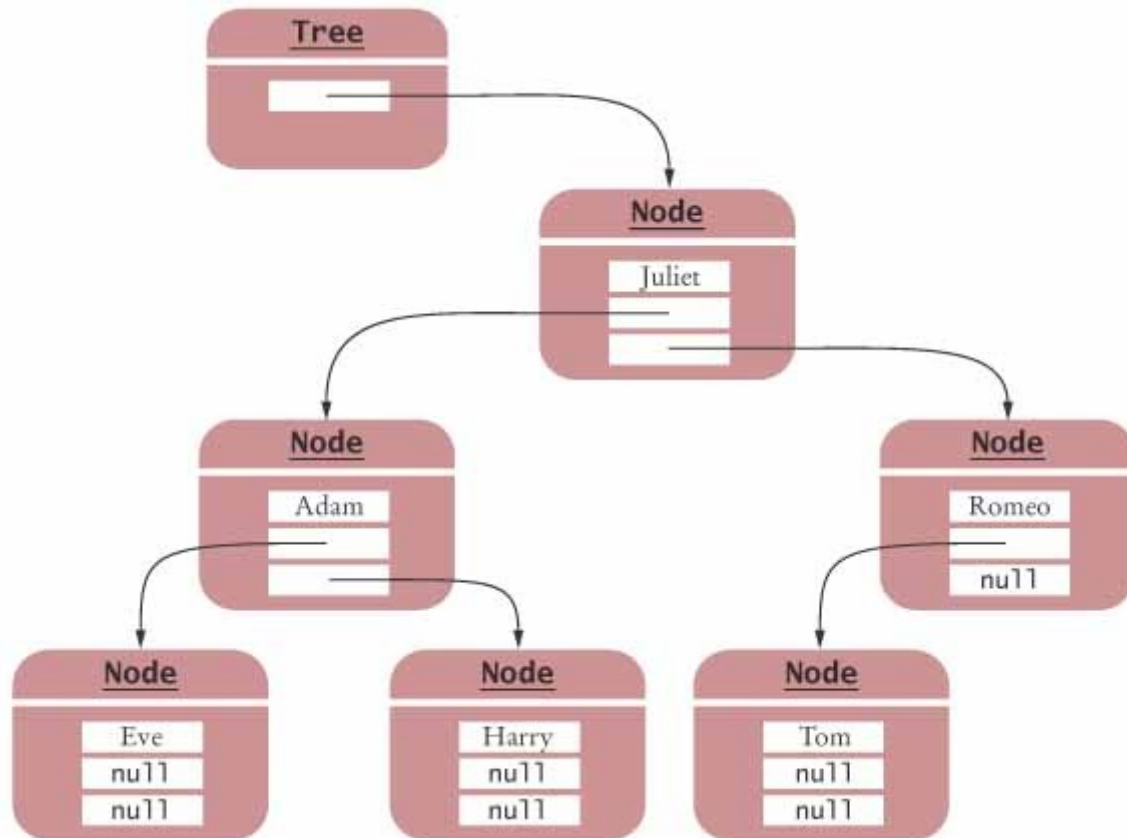
FIGURE 16-8 A Binary Tree That Is Not a Binary Search Tree
