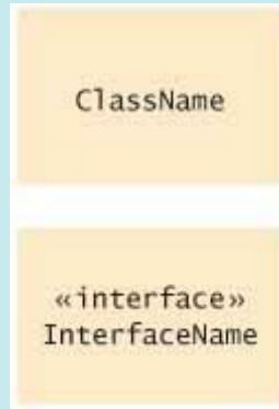
FIGURE M-1 UML Symbols for Classes and Interfaces
