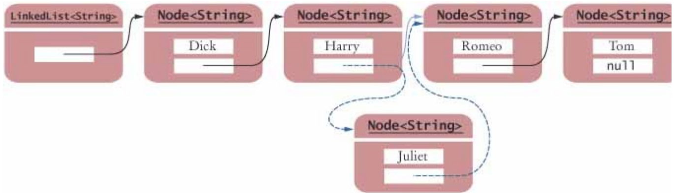
FIGURE 15-1 Inserting an Element into a Linked List
