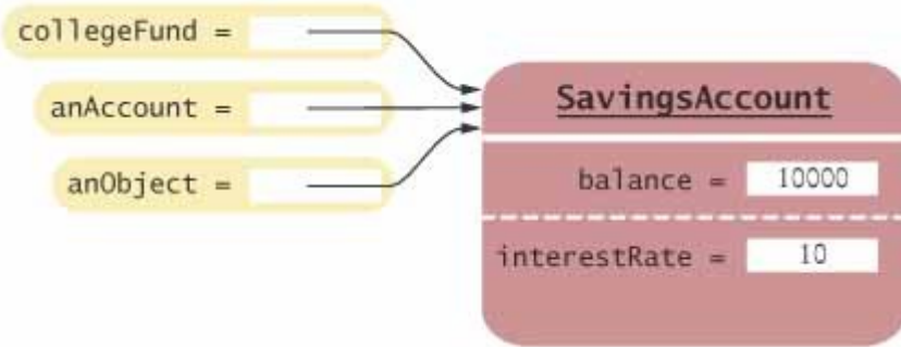
FIGURE 10-7 Variables of Different Types Refer to the Same Object
