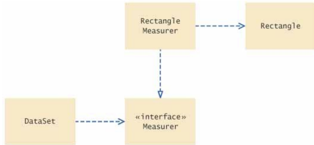
FIGURE 9-2 UML Diagram of the DataSet Class and the Measurer Interface
