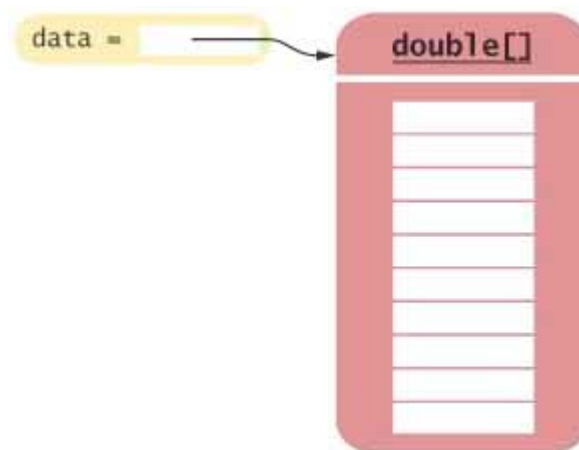
FIGURE 7-1 An Array Reference and an Array
