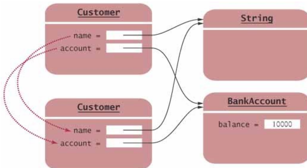
The Object.clone Method Makes a Shallow Copy
