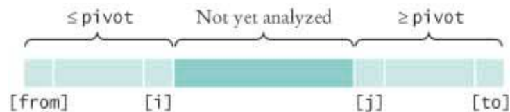
Partitioning a Range
