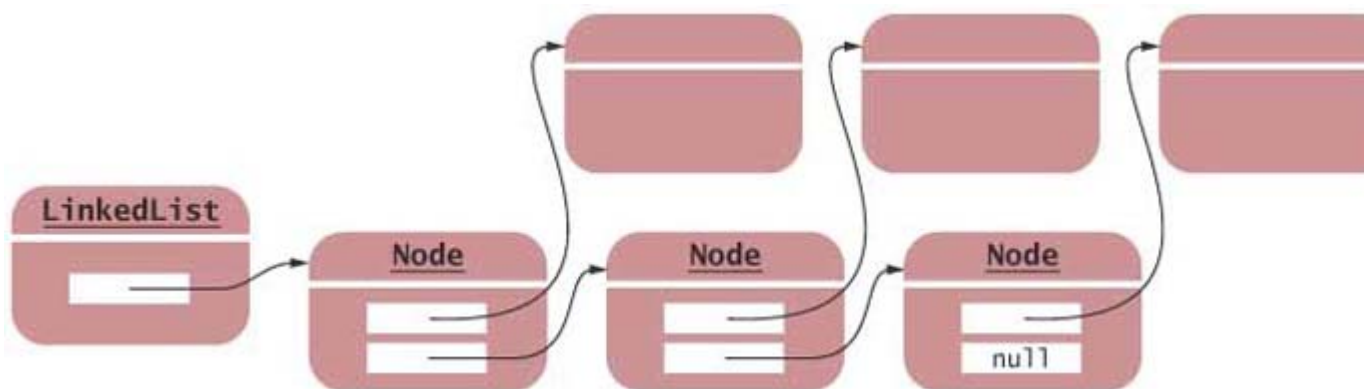
FIGURE 15-8 A Concrete View of a Linked List
