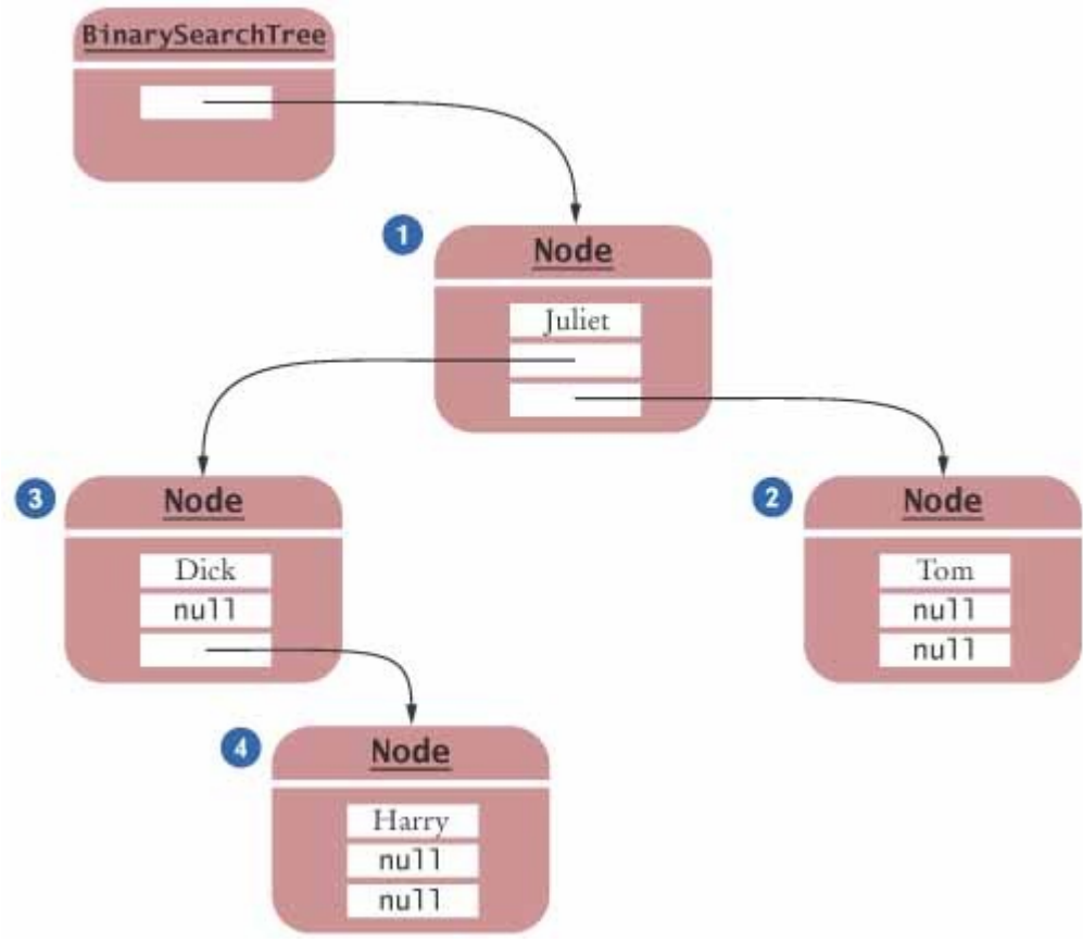
FIGURE 16-9 Binary Search Tree After Four Insertions
