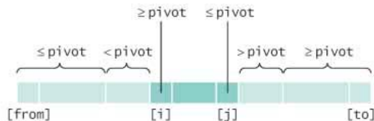
Extending the Partitions
