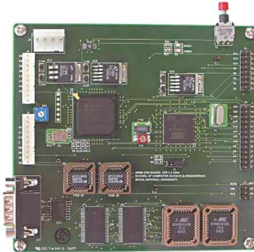
FIGURE 20-4 The Controller of an Embedded System
