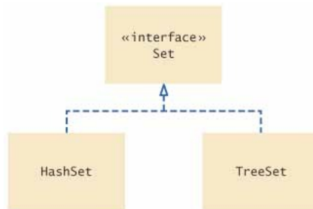
FIGURE 16-2 Set Classes and Interfaces in the Standard Library
