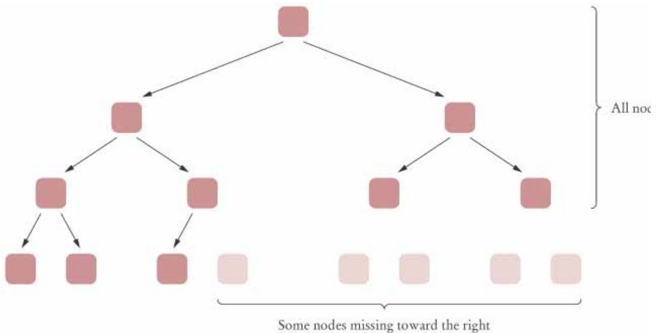
FIGURE 16-16 An Almost Complete Tree
