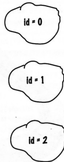
HeapQuiz Objects:
