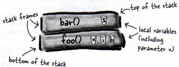
A call stack with two methods
